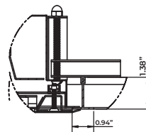
PDR (W/ OC FRAME) RECESSED GRID
