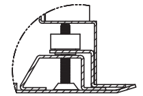
OC FRAME DETAIL
