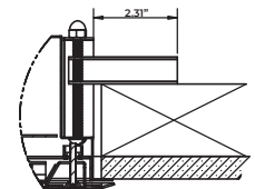
PDR (W/ OC FRAME) RECESSED FLANGE
